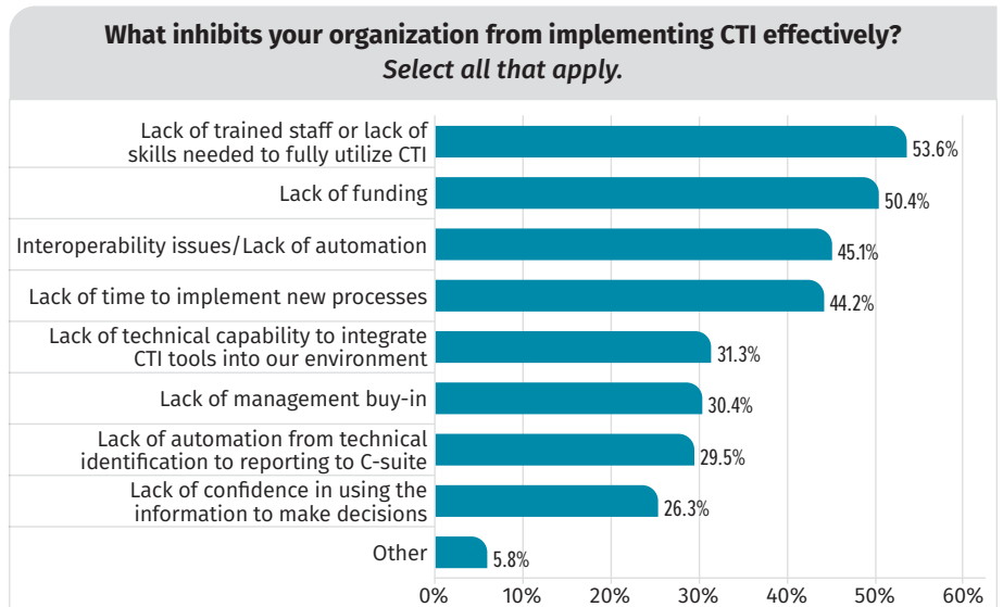
Figure 15. CTI Inhibitors
